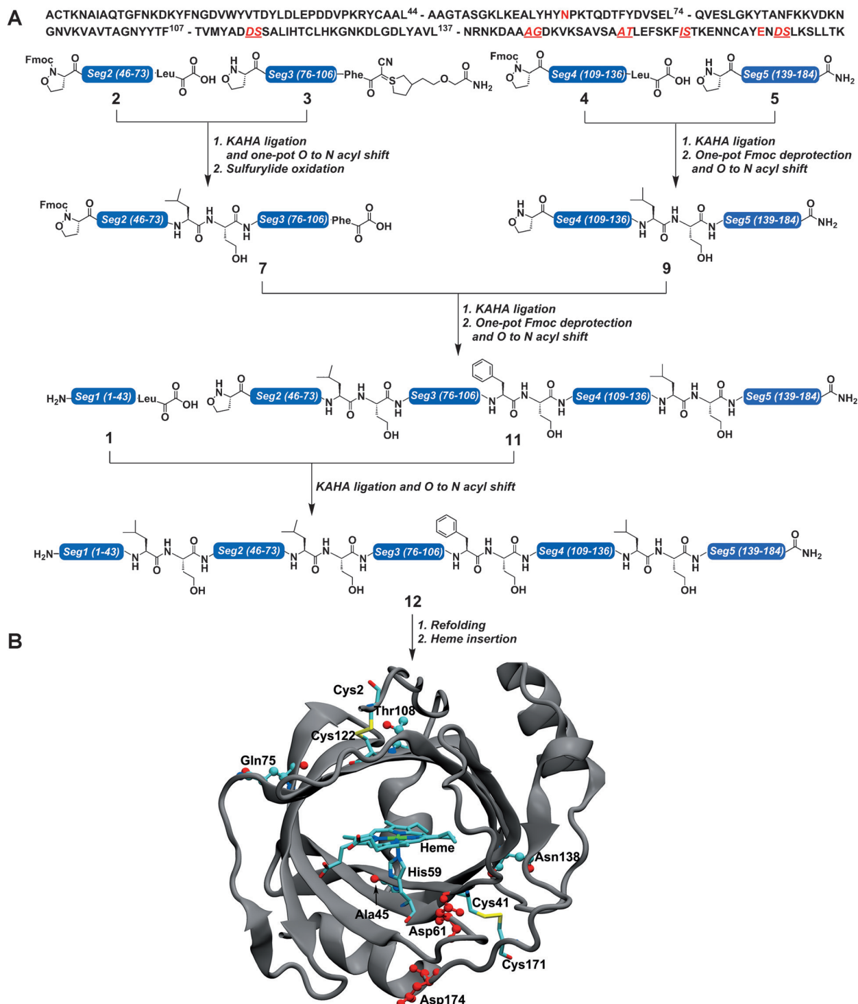
Figure 1. Total chemical synthesis of NP4[T S 45, 75, 108, 138, D61N, D174E]. A) Amino acid sequence and convergent strategy. Dipeptide building blocks used during SPPS are in red and underlined. Two other mutations, introduced during the synthesis, Asn 61 and Glu 174, are highlighted in red. B) X-ray crystal structure of NP4 at pH 7.5 (PDB code: 1NP4), highlighting the four ligation sites (ball and stick representation), two disulfides (stick representation), and two other mutation sites for synthetic purposes (ball and stick representation, red).
